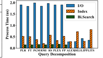
Figure 8: The table (left) reports index performance on three real datasets with the position boundary fixed at 16, while the figure (right) shows the breakdown of a point lookup. LIPP and DILI fail on OSM due to excessive memory requirements (LIPP) and unsupported key distribution (DILI).
