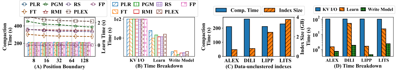
Figure 11: Compaction time, training time, and I/O time. The bars in (A) shows the time of finishing the compaction while the line presents the time used for training the models.
