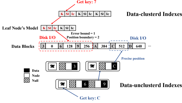
Figure 5: Implementation of two kinds of indexes.
