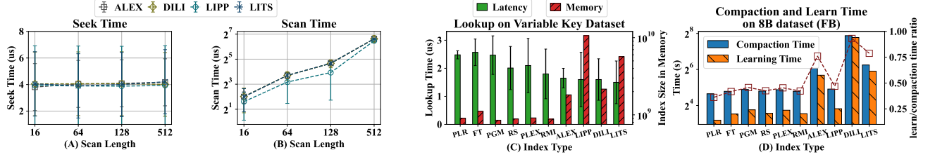
Figure 10: (A) and (B) show range lookup performance of data-unclustered indexes; (C) shows the performance of learned indexes with variable length key lookups; (D) presents the compaction time and learning time under dataset with small key size.
