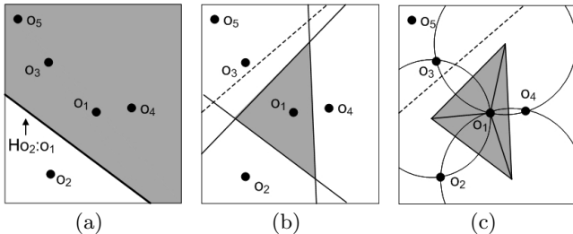
Figure 2: Computing Voronoi cell of o_1
