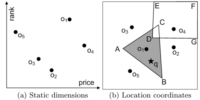
Figure 3: Illustration of safe zone
