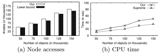
Figure 8: Effect of data cardinality
