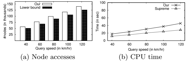
Figure 11: Effect of query speed
