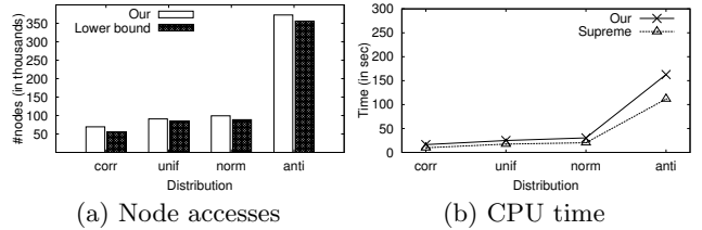
Figure 10: Effect of distribution
