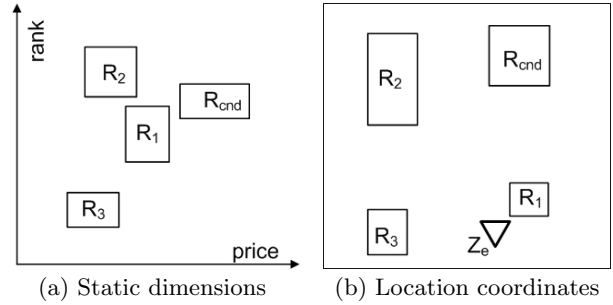
Figure 6: Illustration of pruning
