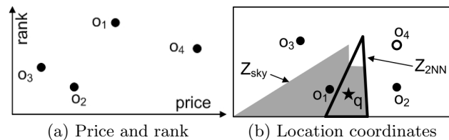
Figure 7: 2-closest skyline objects are o_1 and o_2
