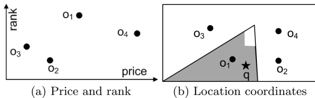
Figure 1: Skyline objects are o_1 , o_2 and o_3 and safe zone is the shaded area
