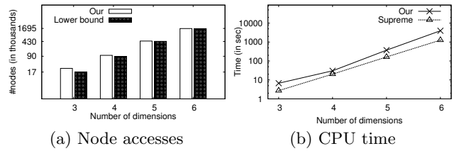
Figure 9: Effect of dimensionality
