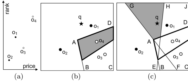
Figure 4: Pseudo Impact Region
