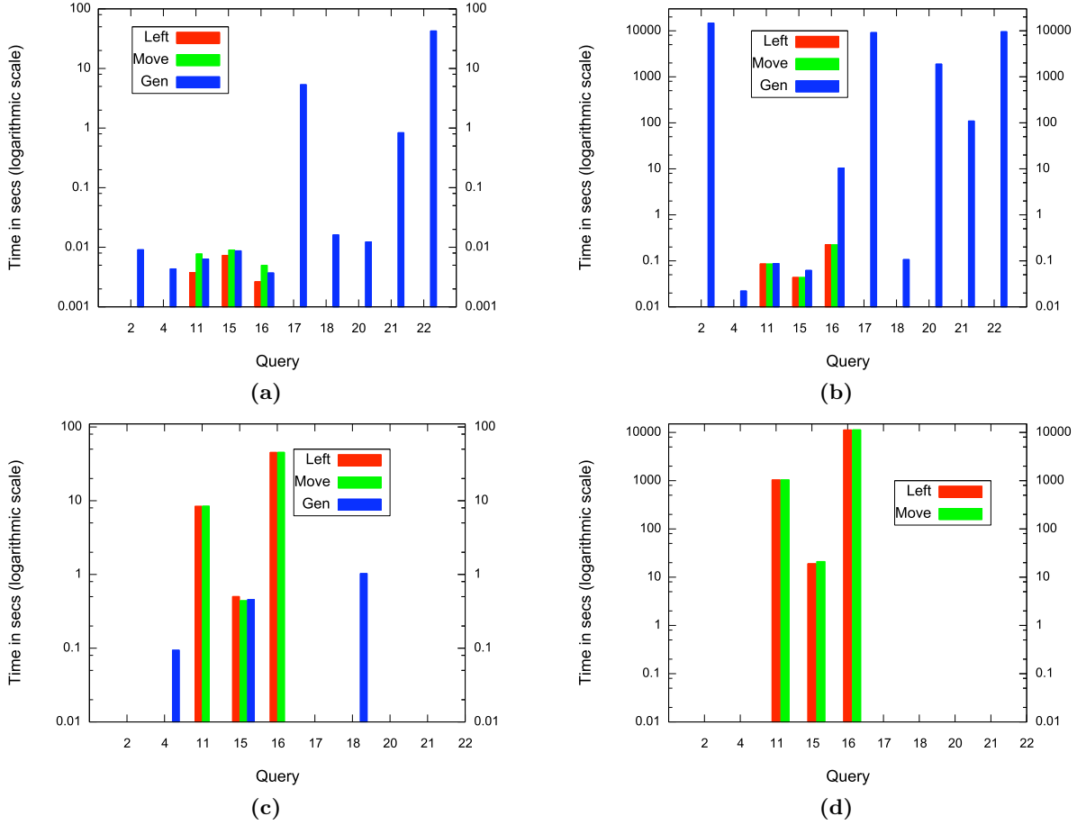
Figure 6: Performance of queries with sublinks in TPC-H for database sizes 1MB (a), 10MB (b), 100MB (c), and 1GB (d)
