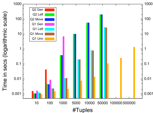
Figure 9: (Synthetic) Varying size of both relations
