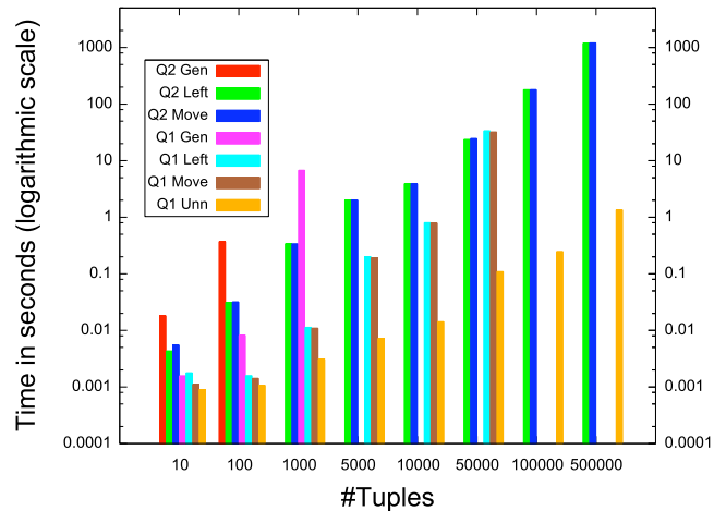
Figure 8: (Synthetic) Varying size of sublink relation
