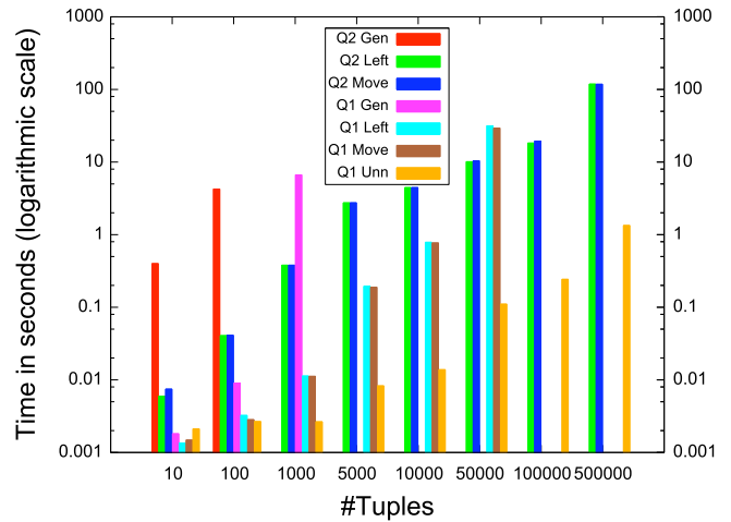
Figure 7: (Synthetic) Varying size of input relation
