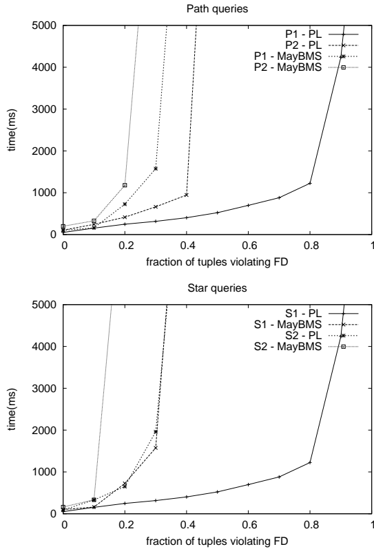
Figure 6: Varying the number of offending tuples.
