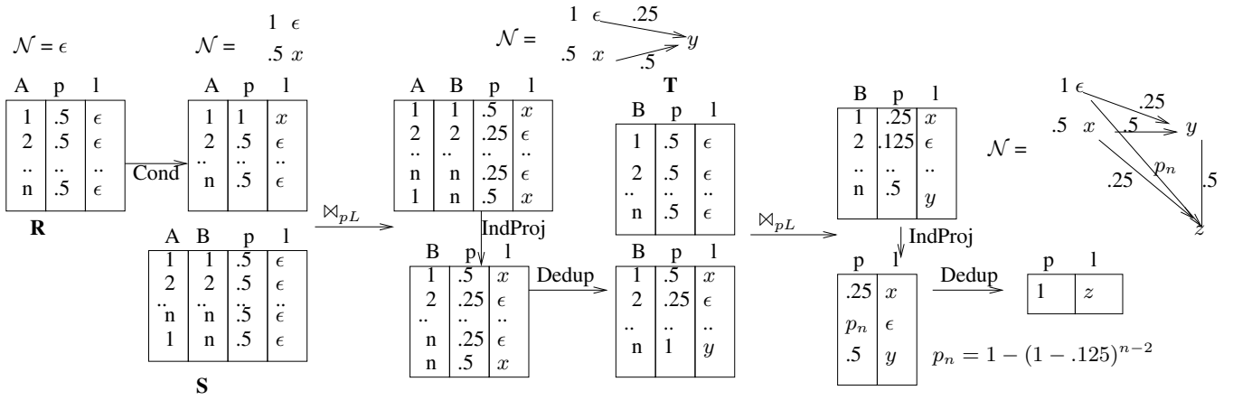
Figure 4: Evaluating q : -R(x)S(x,y)T(y) . Pr(q) is given by \mathcal{N}^0(z = 1) . P values for leaves and edges in \mathcal{N} are written besides them.
