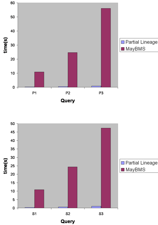
Figure 5: Behaviour for 1% offending tuples.
