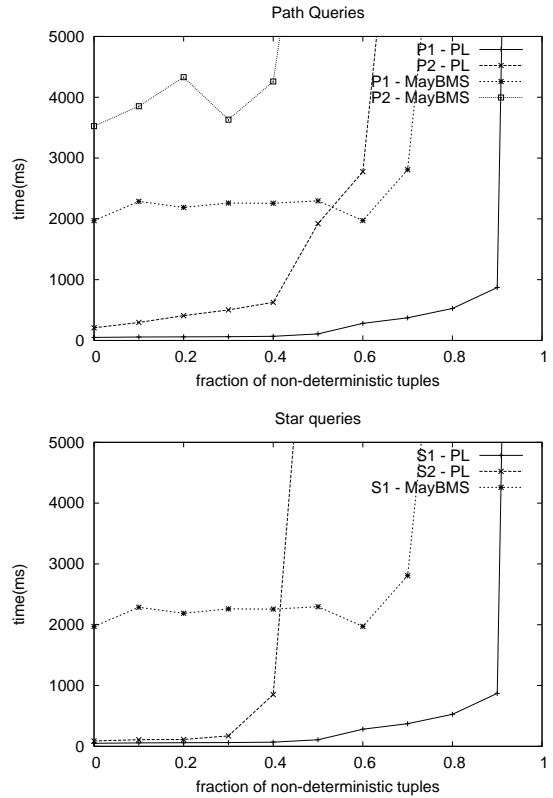
Figure 7: Varying the number of deterministic tuples.
