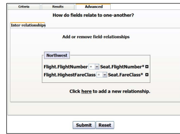
Figure 11: Advanced Pane of the Modified Form
