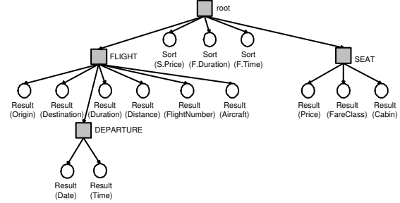
Figure 4: Logical Representation of a Form (Input Tree)
