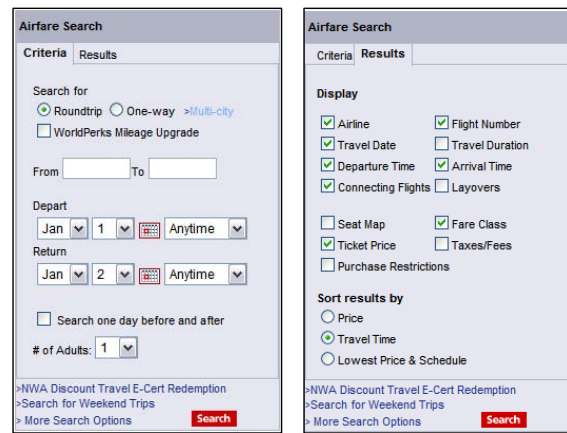
Figure 3: Two-paneled version of Search Form in Fig. 1(a).
